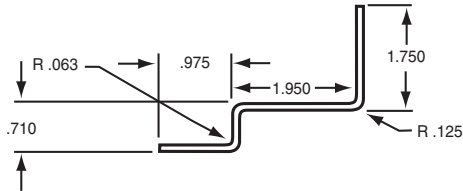
CR-300 For use with Parallel arm closers
