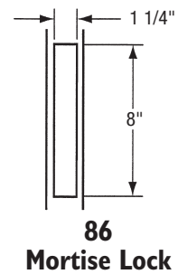
For Use on 1 3/4" Doors
